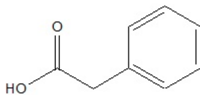
Phenylacetic acid
