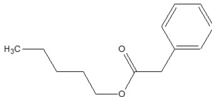
Amyl phenylacetate
